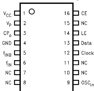
TSSOP 16-Pin Package
